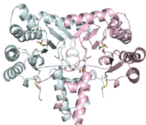
Ribbon Model of NDPS1 from Tomato Homodimer Formed by Binding of 2 Enzymes of the Same Type (Light Blue & Pink)
