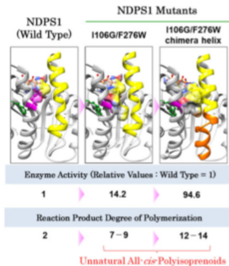
NDPS1 Mutant Structural Models & Properties Comparison
