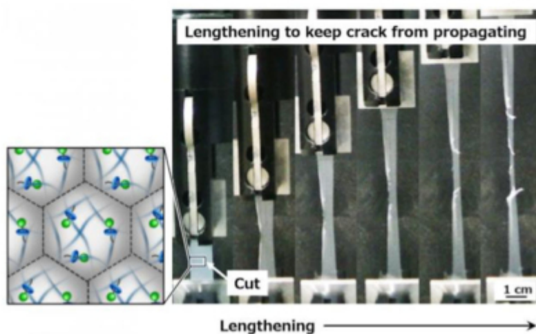
Illustration of a tear test from a cut in a nanoparticle film
